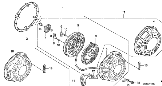
RECOIL STARTER(1)
